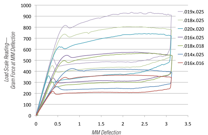
Tooth-Moving Force Characteristics of Elastinol Square and Rectangular Drift-Free Archwires
