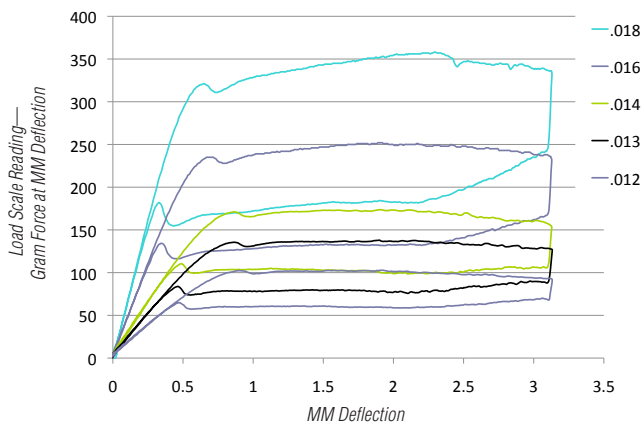
Tooth-Moving Force Characteristics of Elastinol Round Drift-Free Archwires
